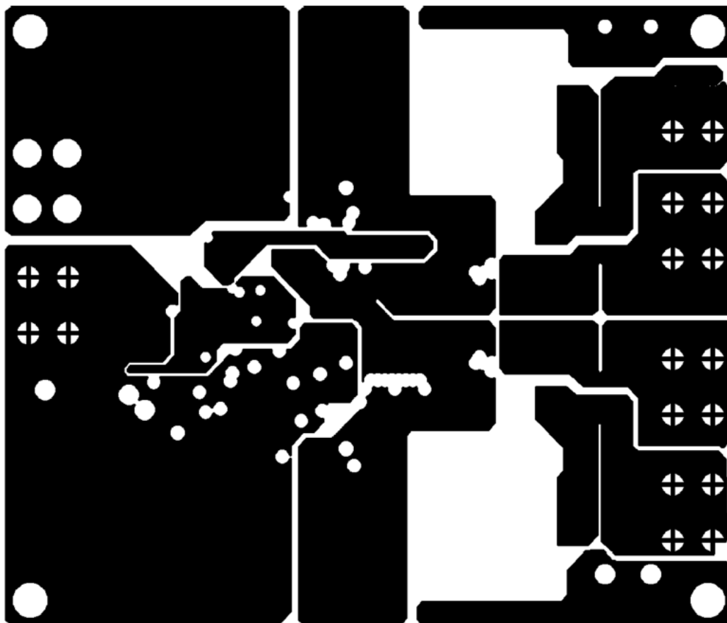
LAYER 2 (.LY2) AS VIEWED FROM TOP
