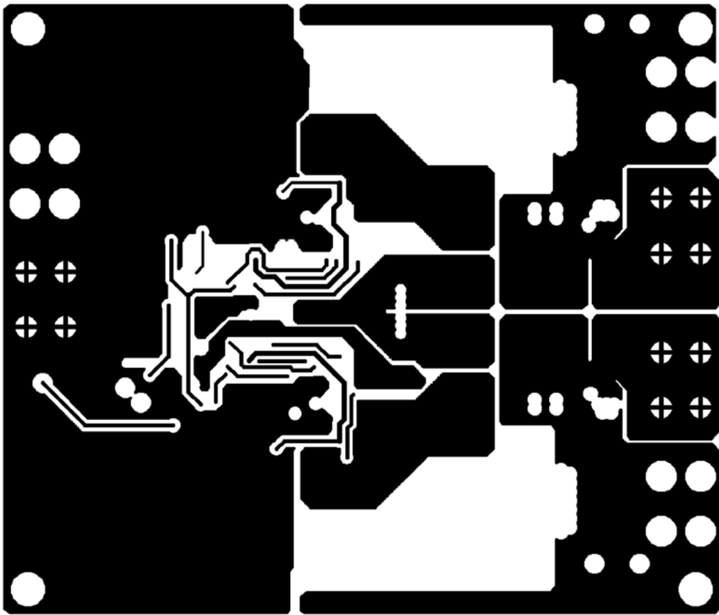
LAYER 3 (.LY3) AS VIEWED FROM TOP
