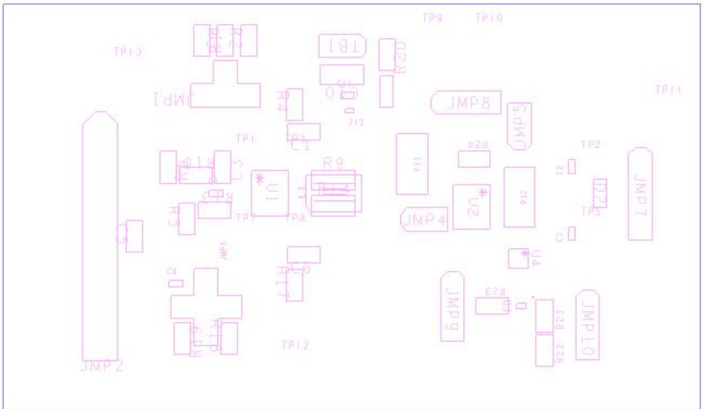
TIDA-01238 CAN Selectable Termination
